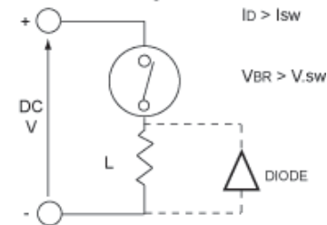
3. DC switching currents
